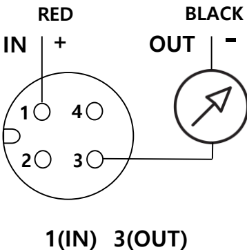
M12*1.0P
