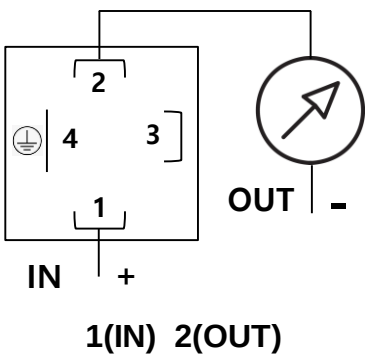
DIN43650C
