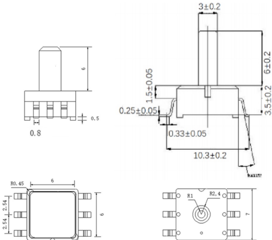
AO100DP SOP6 Top Tube TOL : ± 0.2mm
